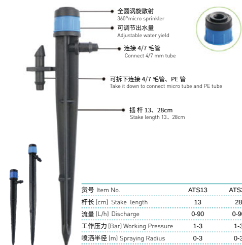
插尖涡旋喷头 Turbo Sprinkler on Stake
