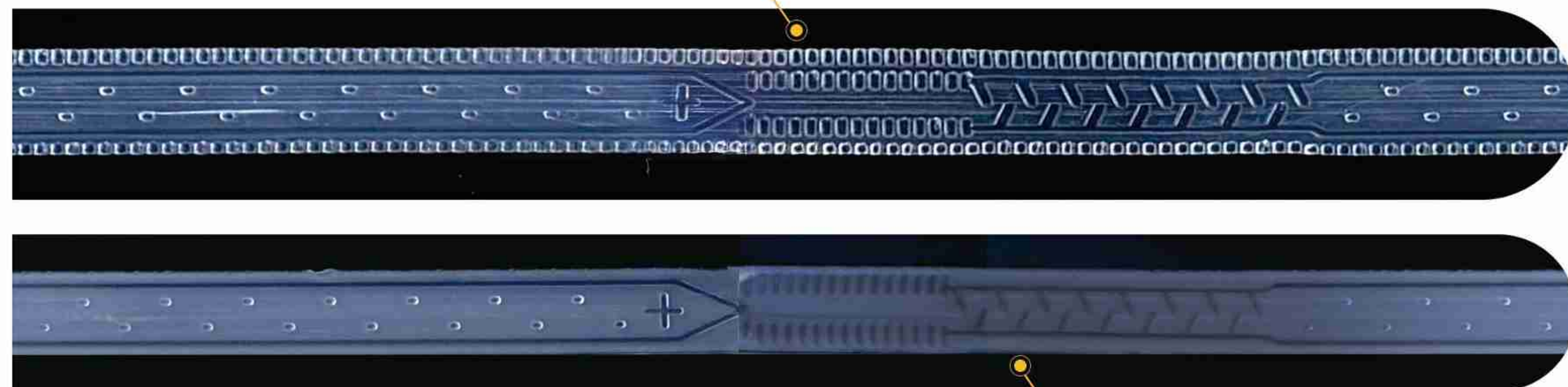
传统内镶连续贴条式滴灌带 Traditional labyrinth drip tape
